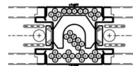
8 Bundles of 4, plus 5 = 41 Cat 6 Cables
