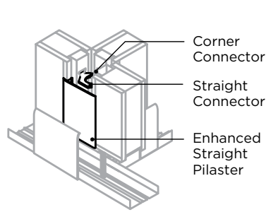
ENHANCED 3-WAY CONDITIONS
