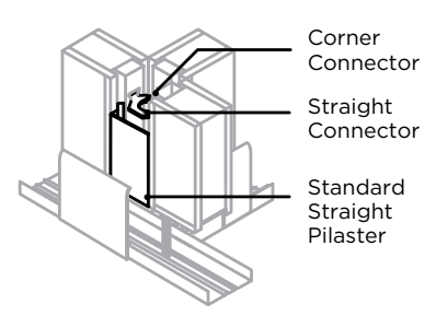
STANDARD 3-WAY CONDITIONS
