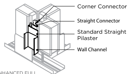
ENHANCED FULL EXTENDED 4-WAY CONDITIONS
