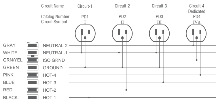
8-WIRE 4-2-2 POWERPAC WIRING DIAGRAM
