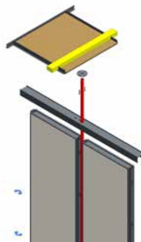
CEILING BRACE FOR PANEL-TO-PANEL CONDITIONS
