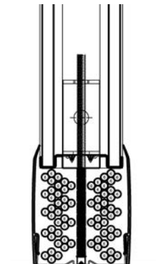
18 Bundles of 4 = 72 Cat 6 Cables
