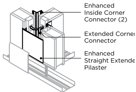
ENHANCED FULL EXTENDED 3-WAY CONDITIONS
